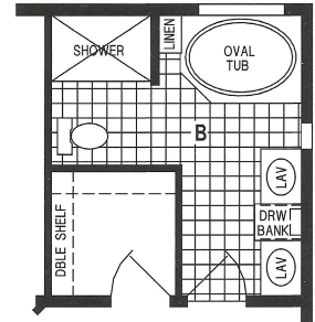
OPTION CORNER OVAL TUB BATH
