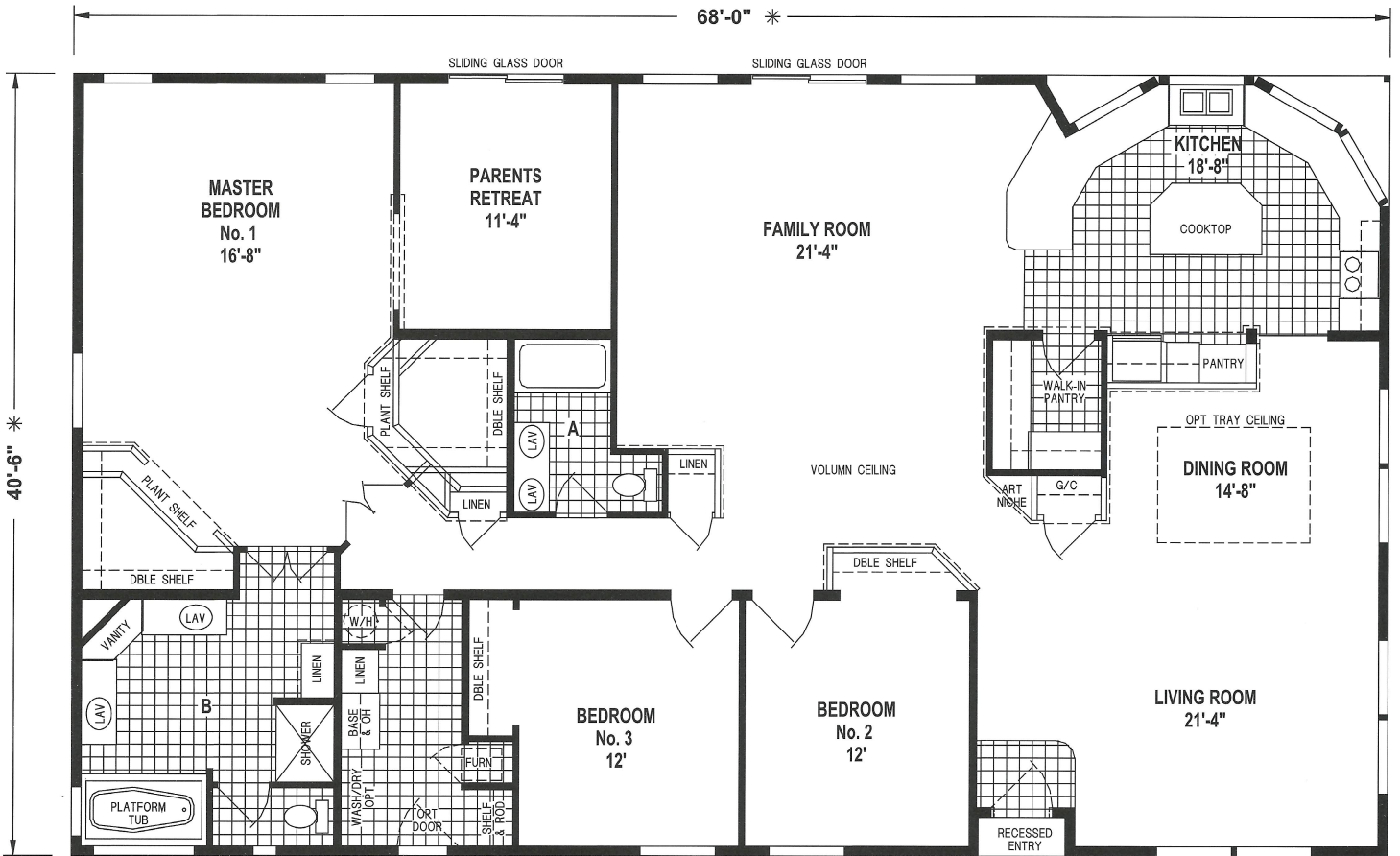
1280CT/6842 (2,720 SQ. FT.) 3BEDROOM - 2BATHS
