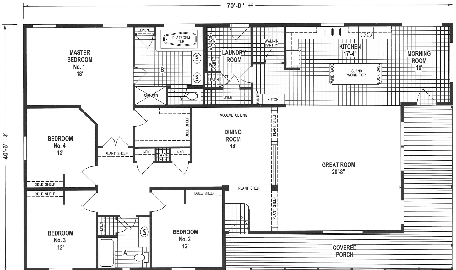
1271CT/7042 (2,444 SQ. FT.) 4BEDROOM - 2BATHS
