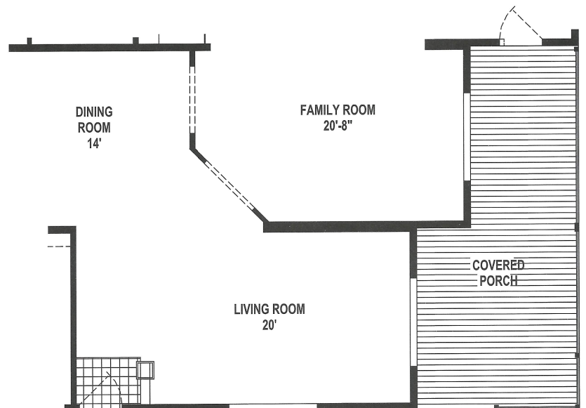
OPTION FAMILY ROOM/PORCH (2,565 SQ. FT.)
